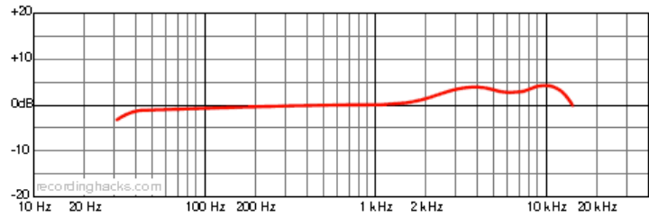
Frequency Response - Cardioid Click Graph to Compare!
